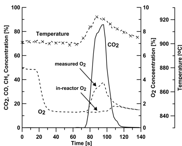
Figure 3.2 Concentration and temperature profiles for C4A-950 during reduction cycle at 900°C.
